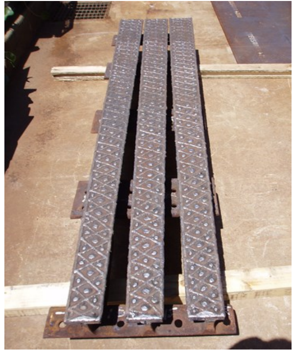
Rock quarry grizzly cassette
